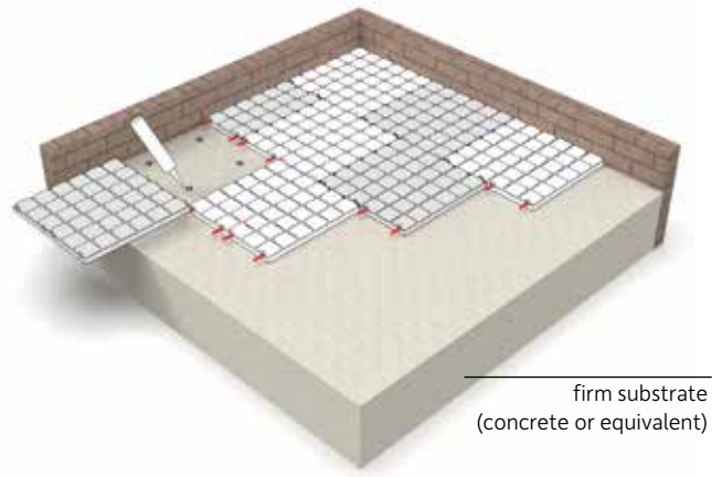
Laying (staggered) on a level, solid surface with system plugs. Bonding with gluing spots on the drainage.
