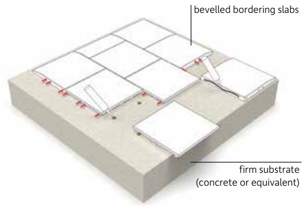
Laying (staggered) on a level, solid surface with bevelled edge slabs & system plugs. Bonding with gluing spots on the drainage.
